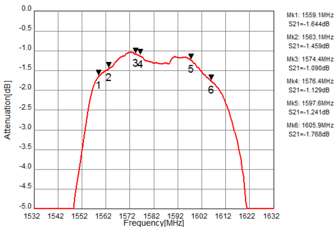
Fig.2 In-band Characteristics
