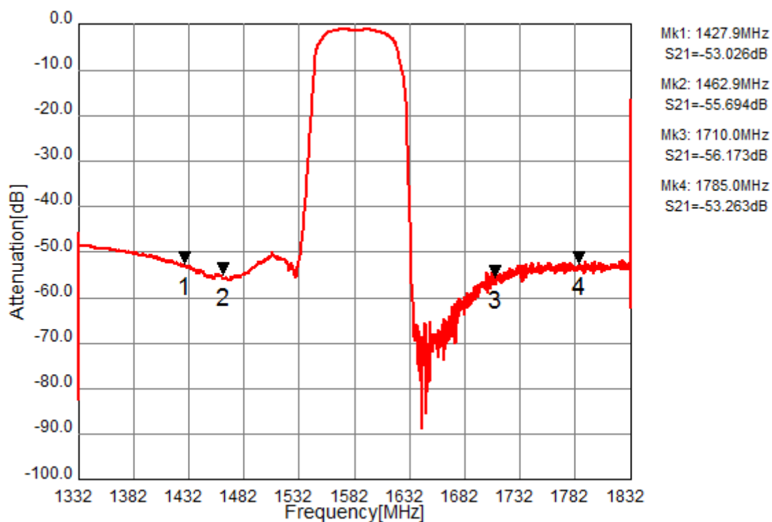
Fig.1 Pass-band Characteristics
